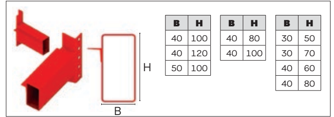
Tumaklı Kutu Travers Box Beam with / nails
