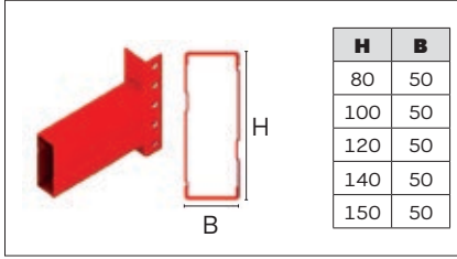
CC Travers CC Beam
