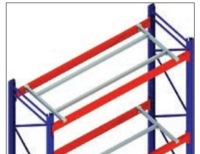
Çiftli H Tipi Travers Double H Type Beam
