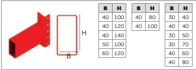
Kutu Travers Box Beam
