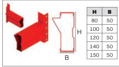
CB Travers CB Beam
